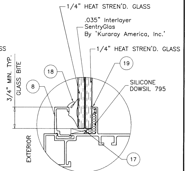
GLASS TYPE 'C' 9/16" OVERALL LAM. GLASS
