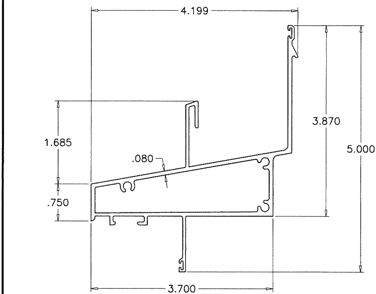
② INTERMEDIATE SILL
