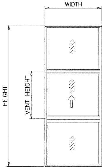
SINGLE HUNG OVER FIXED WINDOWS
