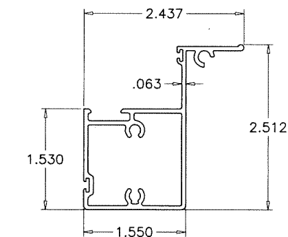
⑥ VENT BOTTOM RAIL
