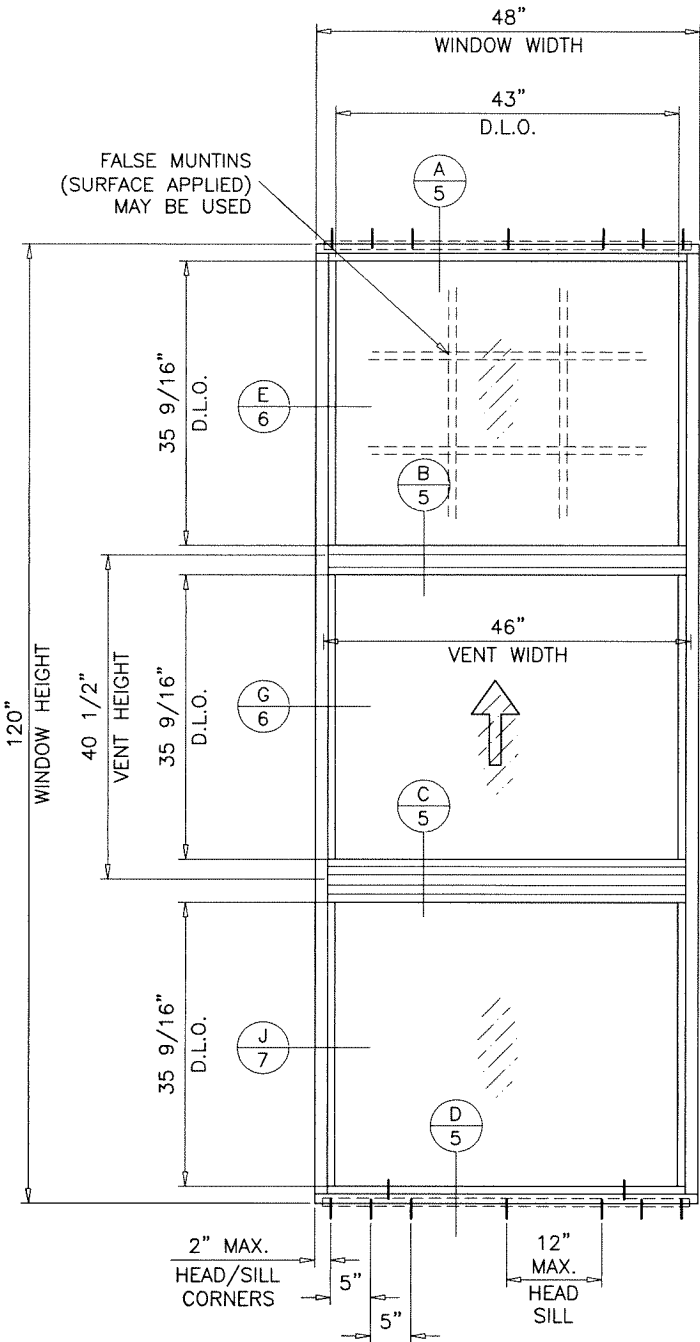
TYPICAL ELEVATION
