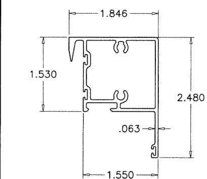
④ VENT TOP RAIL
