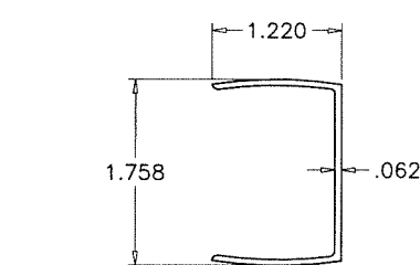
⑬ VENT STOP & VERTICAL COVER
