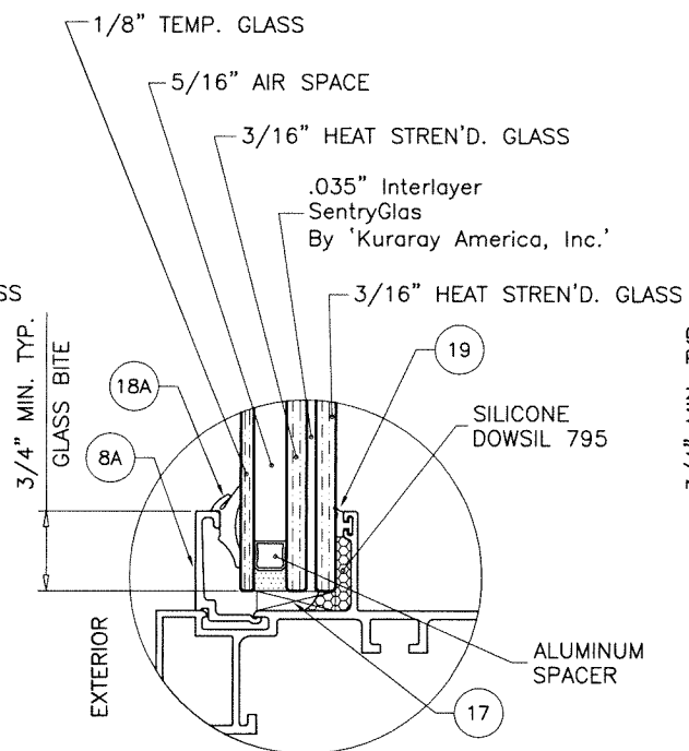
GLASS TYPE 'Bi' 7/8" OVERALL INSUL. LAM. GLASS
