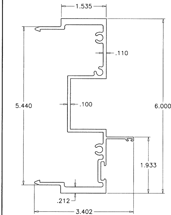
⑨ MALE MULLION
