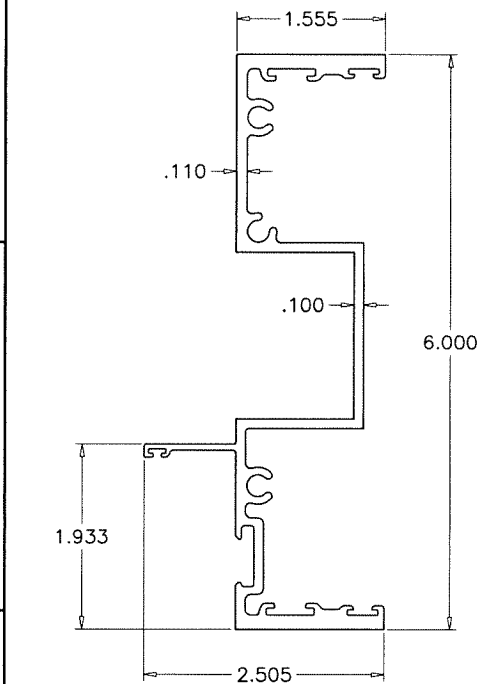
⑩ FEMALE MULLION
